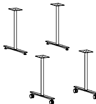
T-Leg Static Base Assembly Kits with Glides and with Casters (See Details)
